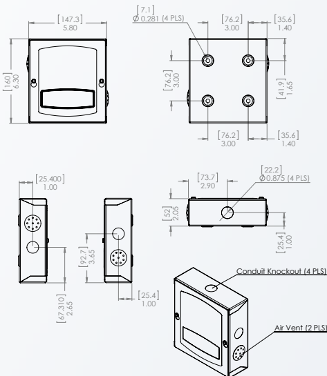
K-O2 with screw cover
