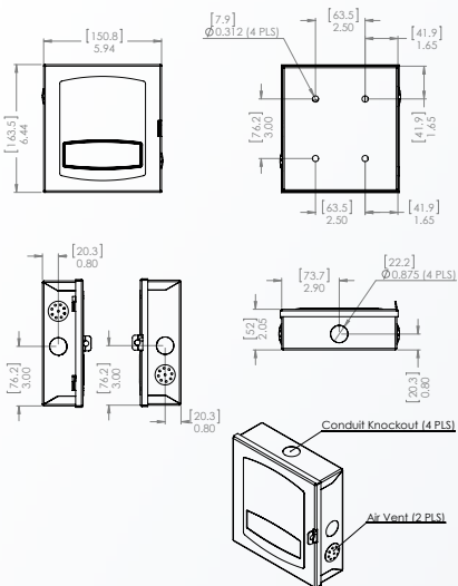
K-O2 with hinged cover
